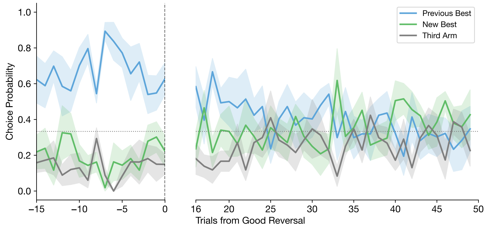
Good Reversal-Aligned Choices (mean \pm se across subjects | n=6 subjects, n=29 reversals) (Skipping first 15 trials post-reversal)
